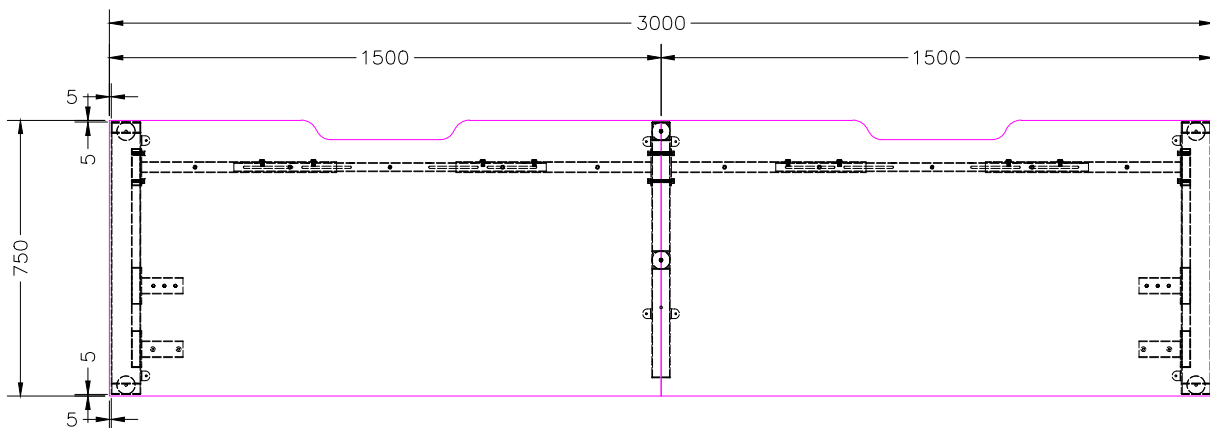
TOP VIEW
