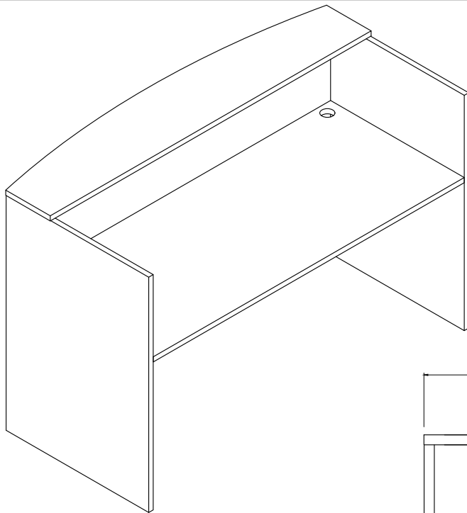
ISOMETRIC VIEW
